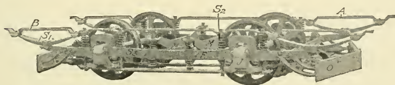
Fig. 9. Brill Single Truck
